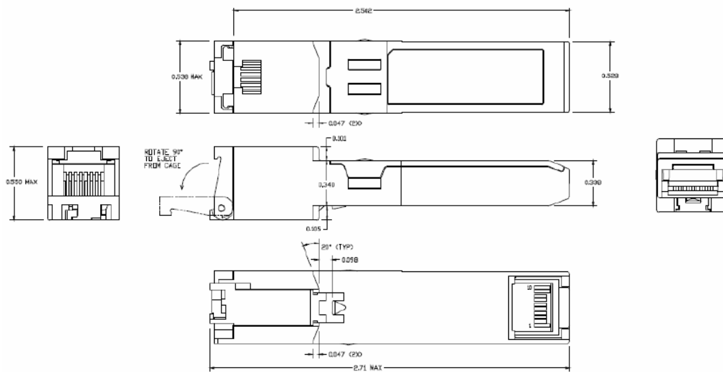
Figure 2. AP-STx mechanical dimensions
