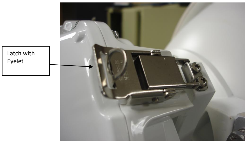
Figure 26 Latch
