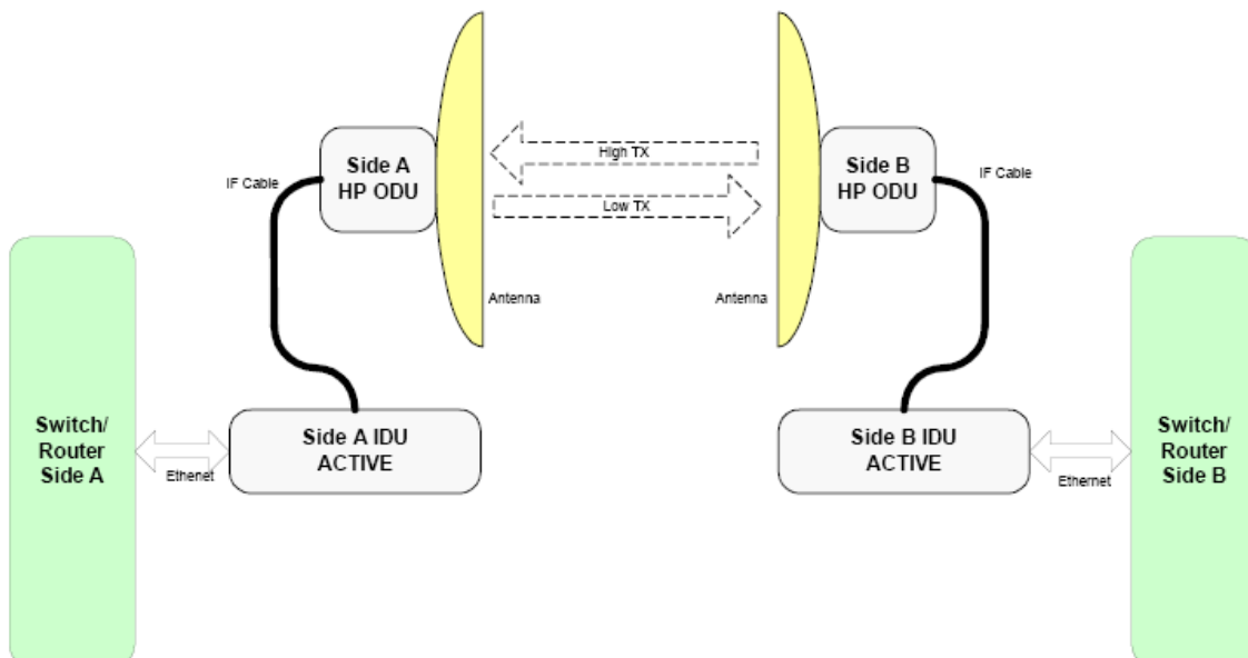
Figure 10 1+0 Setup
